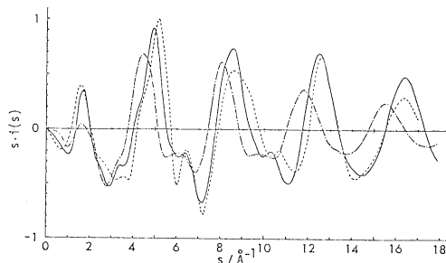
Fig. 1 s_i(s) curves for molten SiO_2 —: X-ray diffraction; ----: MD with the present pair potentials; - · - ·: MD with the pair potentials by Woodcock et al.
