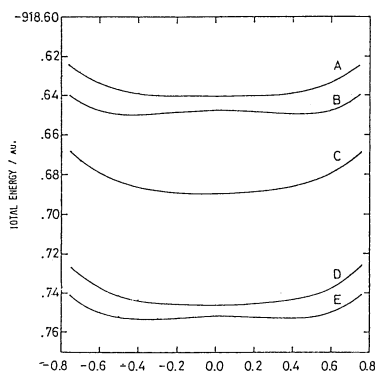
Fig. 1. PROTON DISPLACEMENT VALUE FROM THE CENTRAL POSITION. A - 4-31G SCF, B - 4-31G ** SCF, C - 4-31G CI (basis. 1326), D - 4-31G CI (basis. 3521), E - 4-31G ** CI (basis. 3521), in au.
