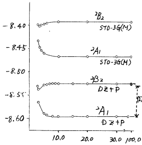
図1. (1): Exp. value of excitation energy
