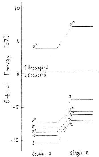
Orbital energy level diagram of DRTC with L=H 2 O (closed-shell RHF)
